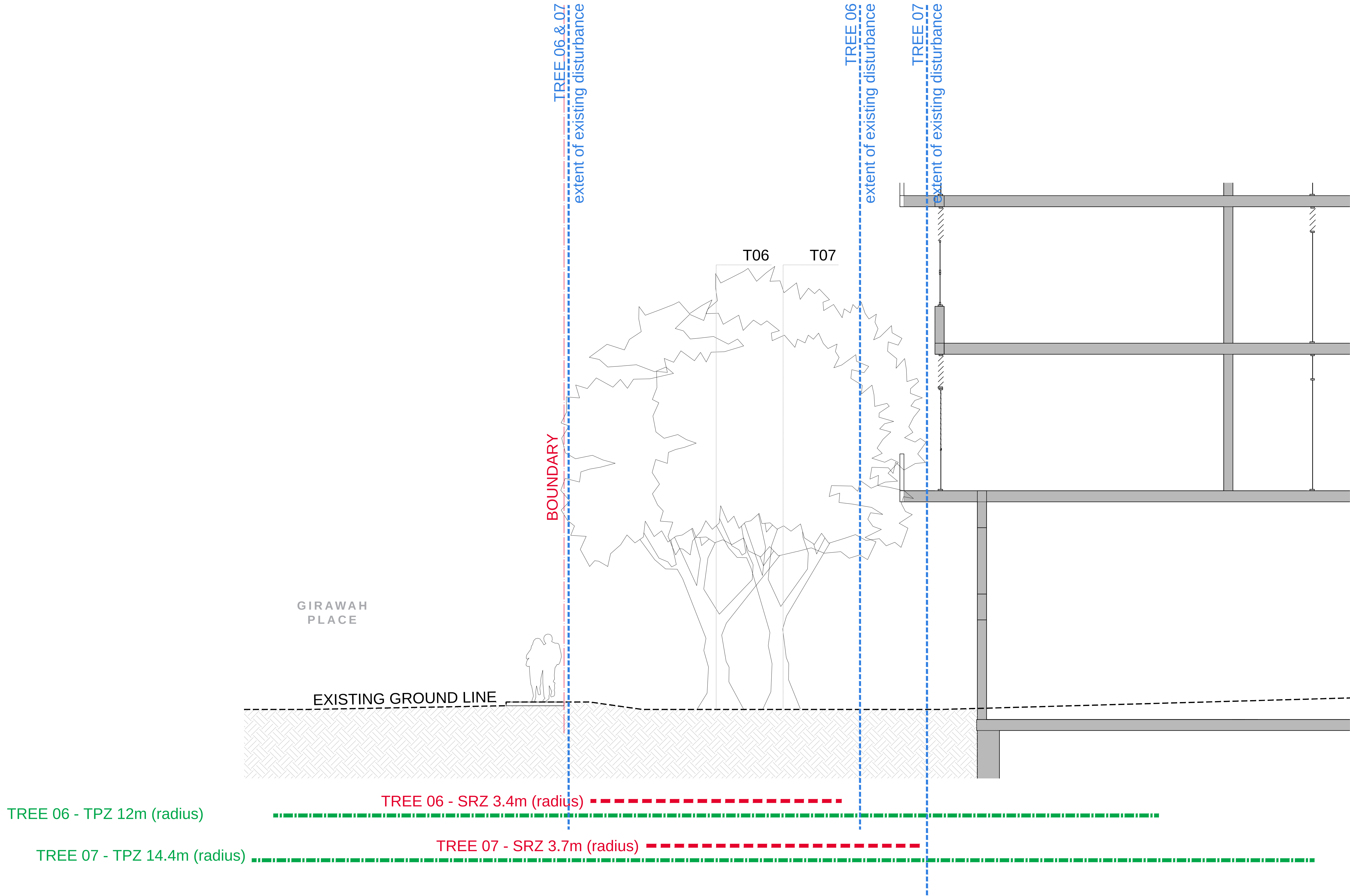
SECTION 1 - 1 Girawah Place Existing trees streetscape section
